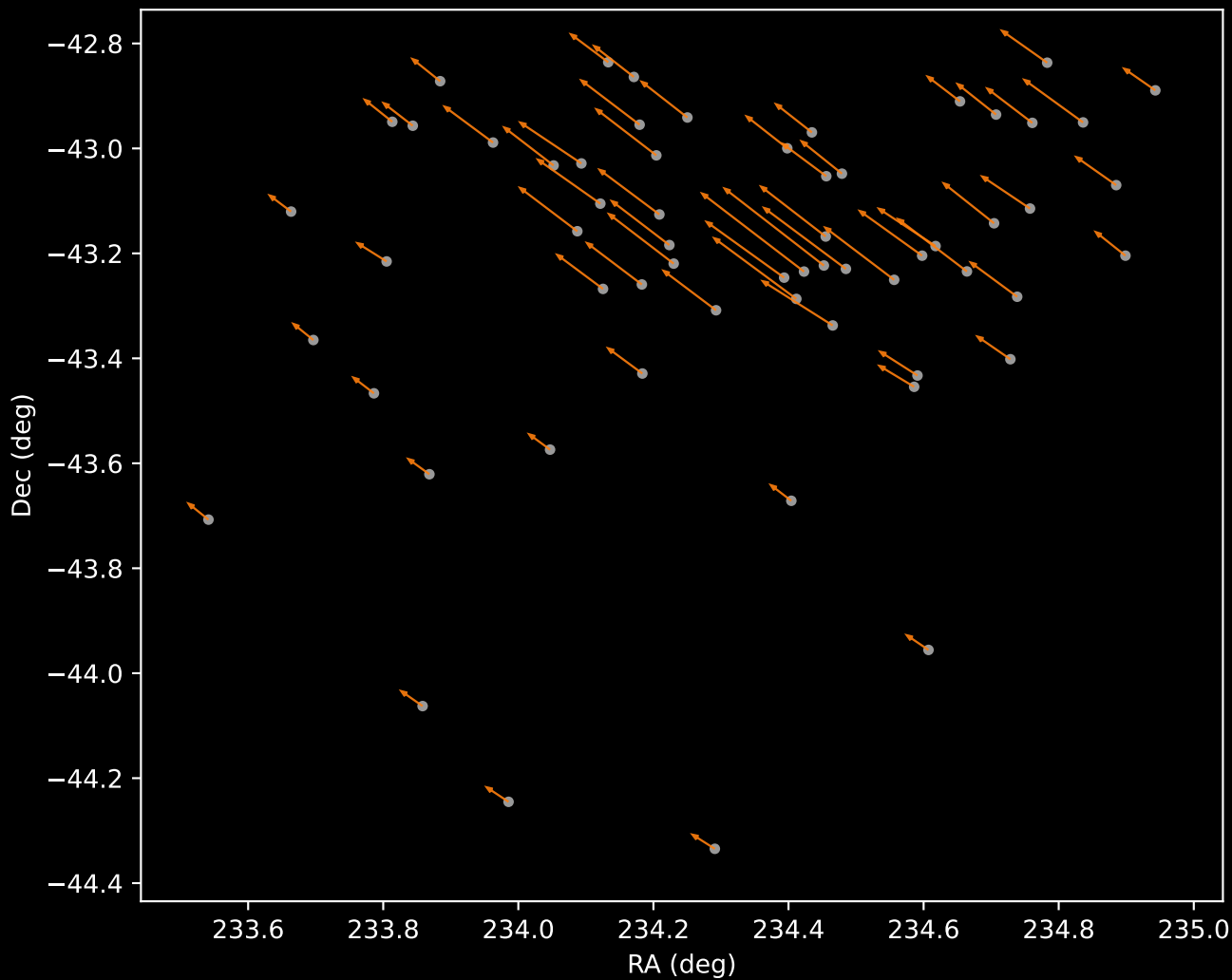
APOGEE DR17 Cluster 2 Proper Motion Vectors (n=61)
