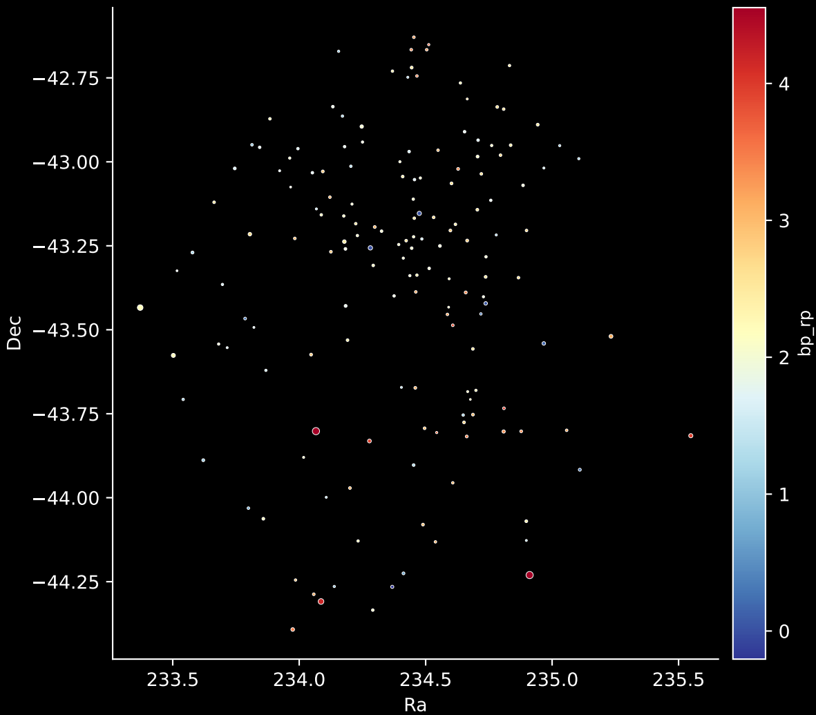
APOGEE DR17 Field: [265+01-C] Stars: 159
