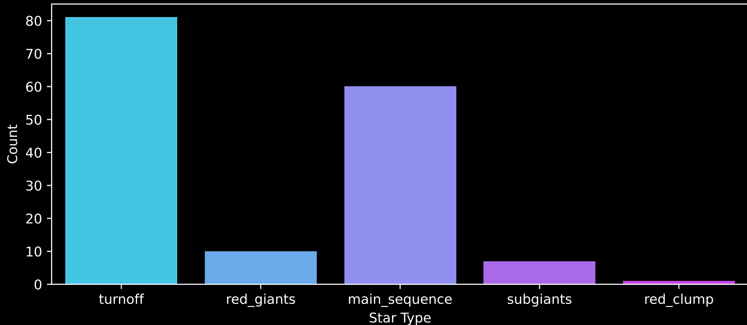
APOGEE DR17 Field: [265+01-C] Count plot of Star Type
