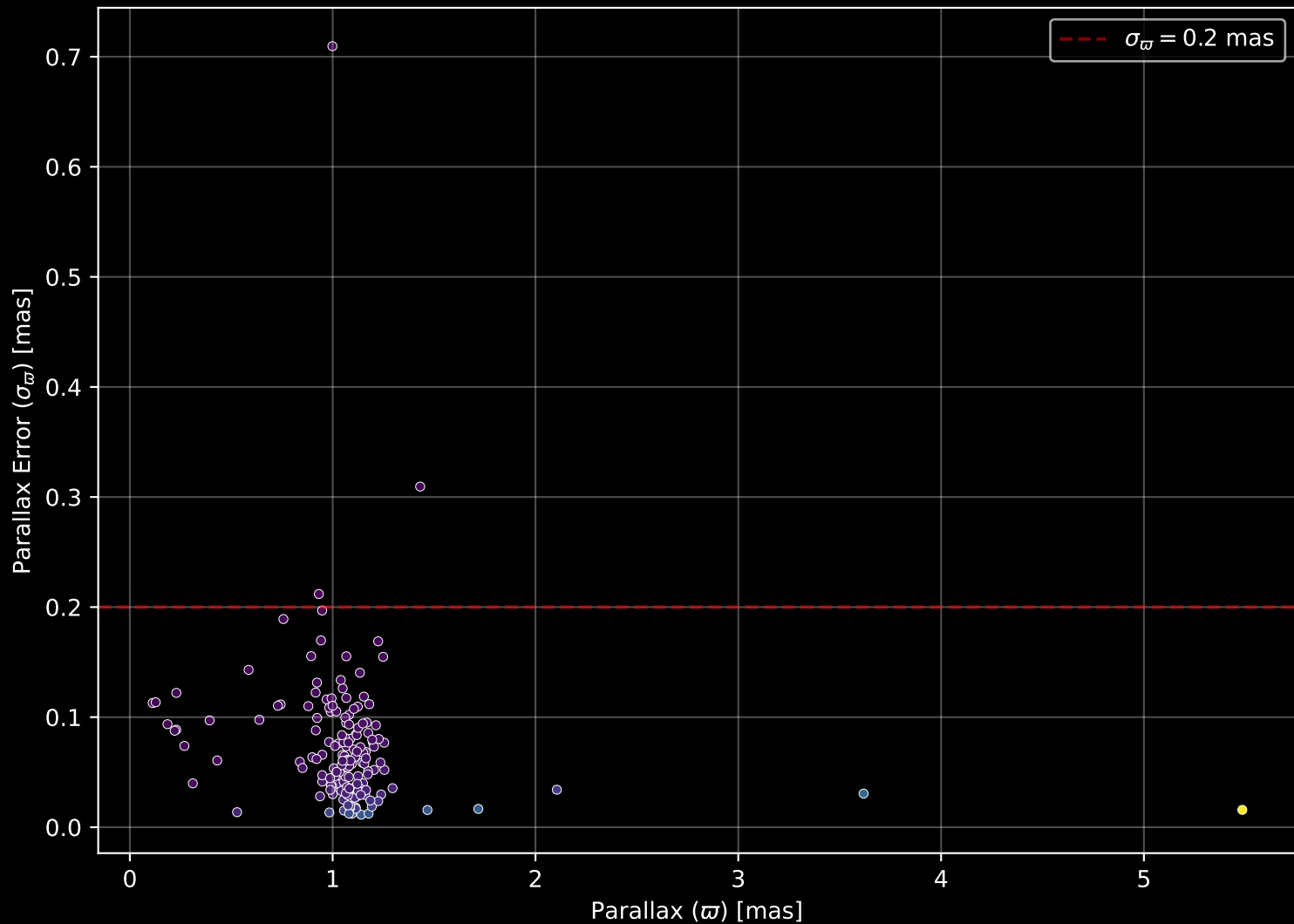
APOGEE DR17 Field: [265+01-C] Parallax Quality (n= 159)
