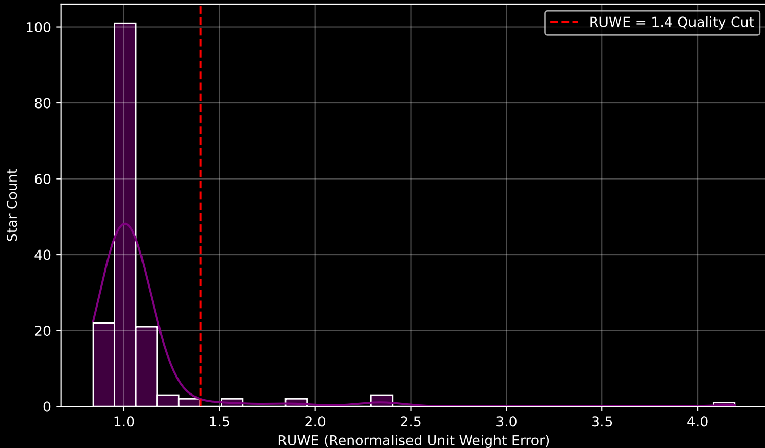
GAPOGEE DR17 Field [265+01-C] RUWE Distribution (n= 157)
