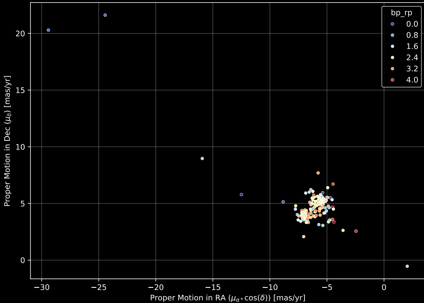
APOGEE DR17 Field: [265+01-C] Proper Motion Diagram (n= 159)
